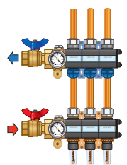
All circuits facing upwards
