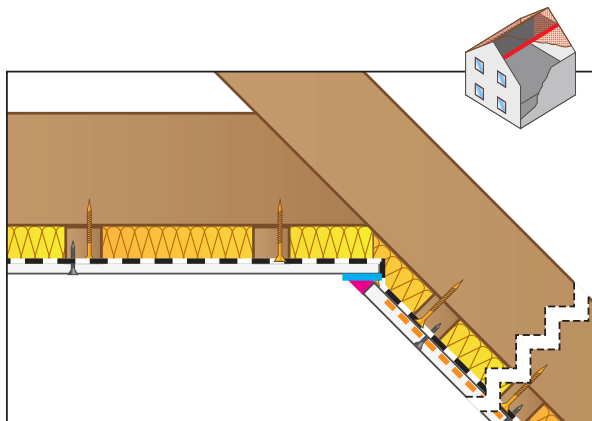
▲ Pitched roof to ceiling
