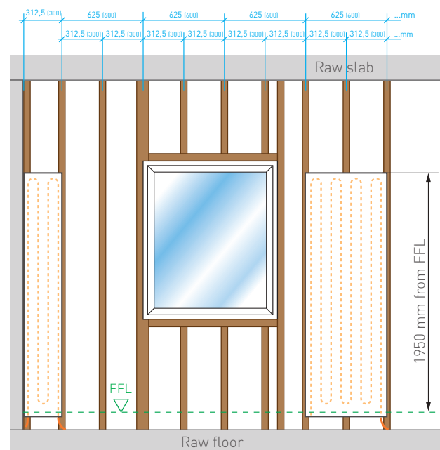
▲ Example of wooden stud construction
