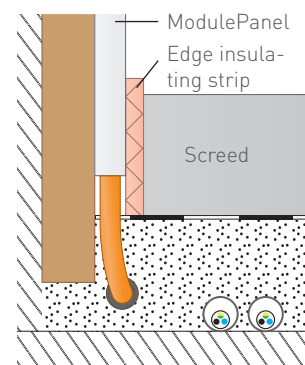
▲ Example cross-section
