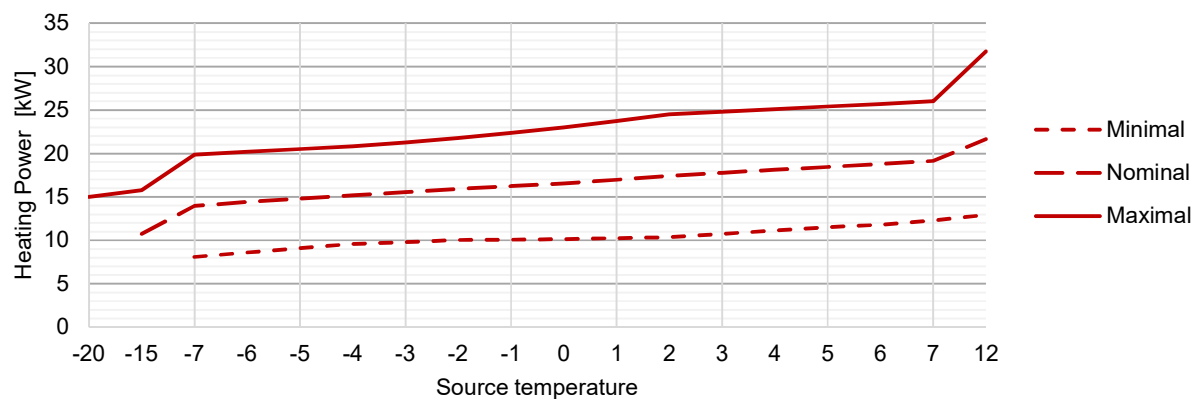
Heating Power WPLT1234 at Flow temperature 55°C*
