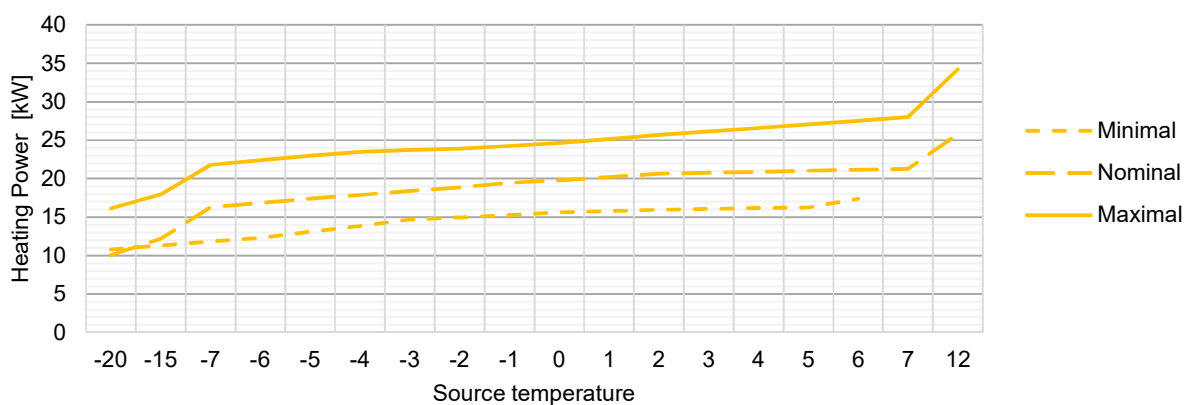
Heating Power WPLT1234 at Flow temperature 35°C*
