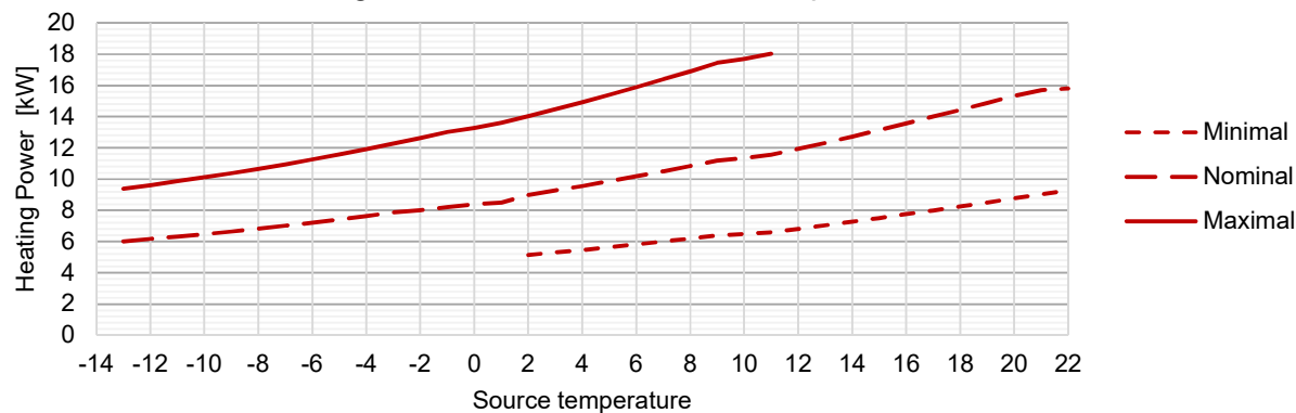
Heating Power WPLK618 at Flow temperature 55°C*
