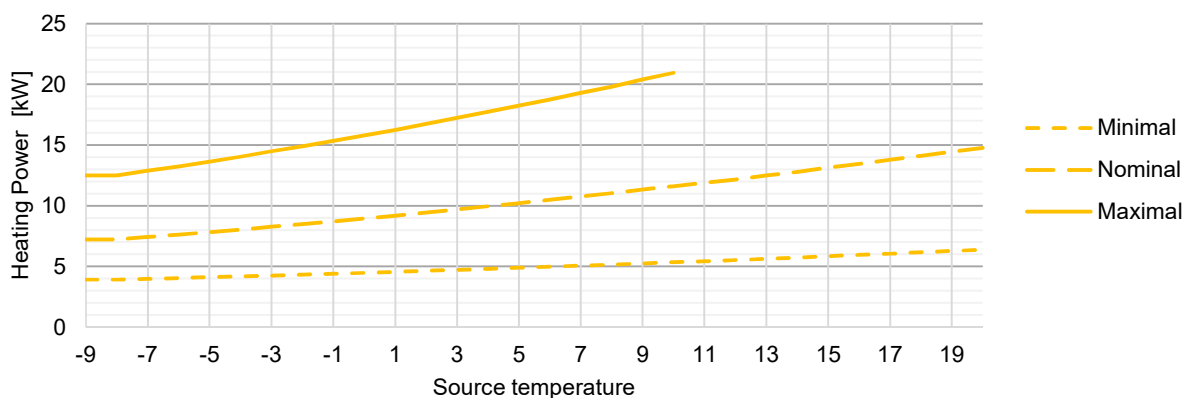
Heating Power WPS618 at Flow temperature 35°C*
