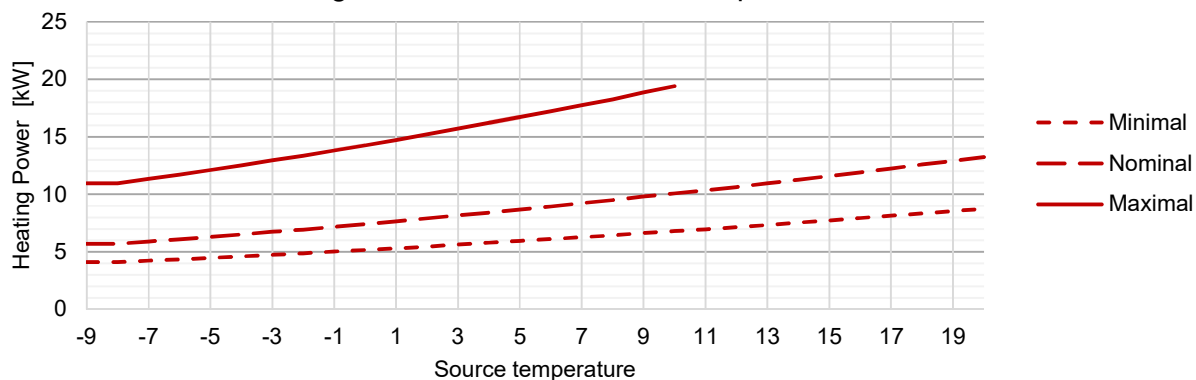
Heating Power WPS618 at Flow temperature 55°C*
