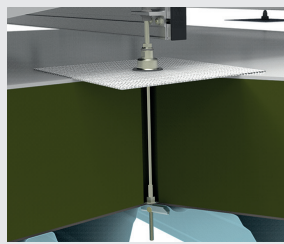
Warm roof TRAPEZ
