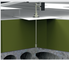
Warm roof CONCRETE
