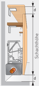
Change in shaft height
