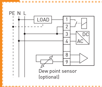
Connection diagram
