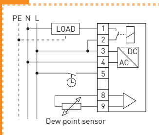
Connection diagram
