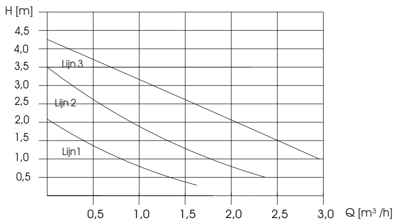
Fabr.: WILLO Type: EAS 25/4-
